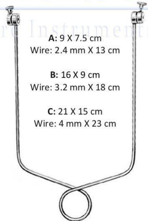
11-01-0435 Bohler Extension Bow for femur & knee
